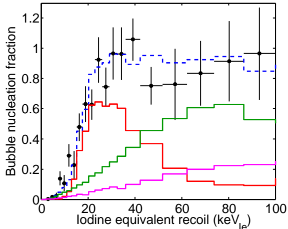
FIG. 2. (Color online) The fraction of pion scattering events that produced bubbles as a function of iodine equivalent recoil energy. The solid curves show the simulated contribution from individual recoil species (from high to low at 20 keV, red for iodine, green for fluorine, and pink for carbon and inelastics), with the blue dashed curve showing the sum. The iodine curve shown takes a step function efficiency model for iodine recoils using the best fit threshold of (16.8_{-1.1}^{+0.8}) keV.
