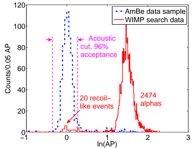
FIG. 2: (Color online) Data from a 553 kg-day WIMP search, shown as a distribution in \ln(AP) in red. Twenty single nuclear recoil events candidates and 2474 alpha events were observed. The blue histogram shows the identical analysis for data taken in the presence of an AmBe neutron source. We define an acoustic cut of 0.7 < AP < 1.3 to select nuclear recoils with an acceptance of 95.8% as determined by the AmBe calibration.
